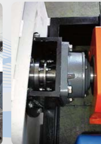
Supporto tenuta Seal and bearing
